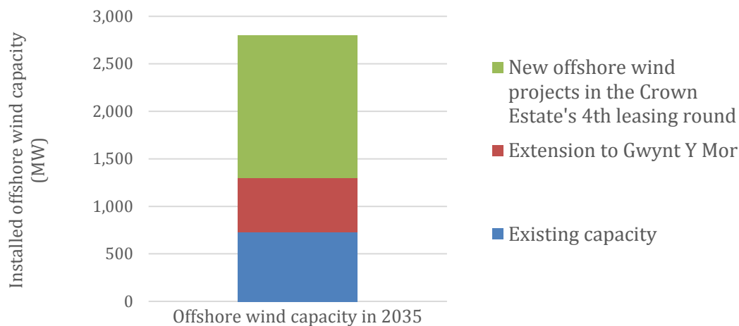
Figure 28: North Wales' Energy Vision scenario for offshore wind. Source: WGES analysis
