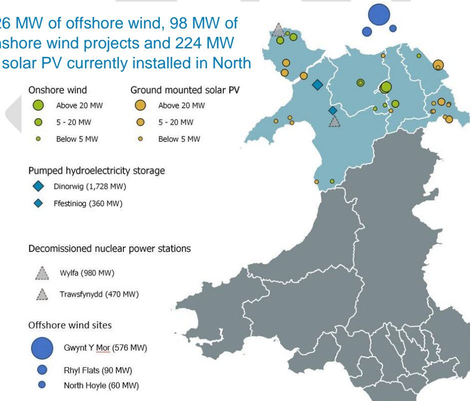
Figure 22: Offshore wind, solar PV and onshore wind projects (>1MW) currently generating in Wales. Source: BEIS Renewable Energy Planning Database, 2019
